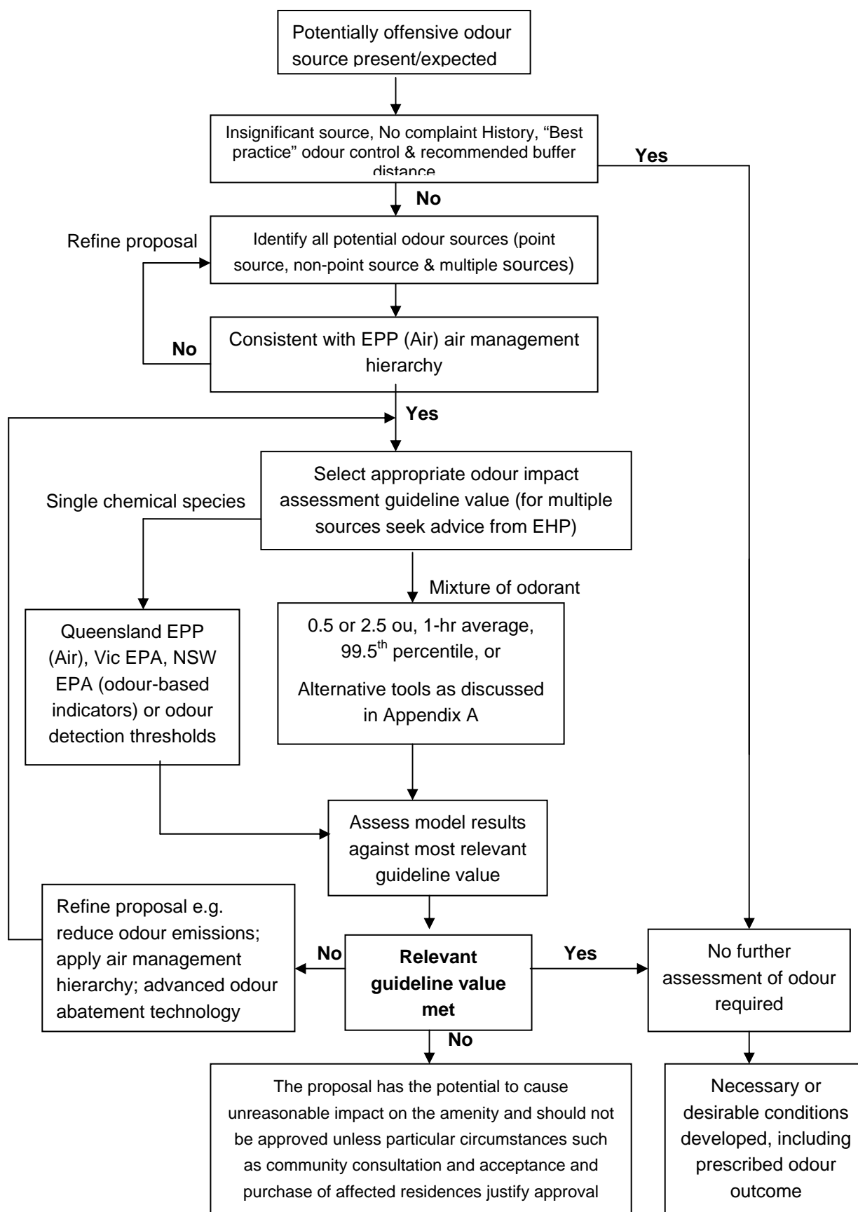
Figure 1. Odour assessment flowchart for new developments.
