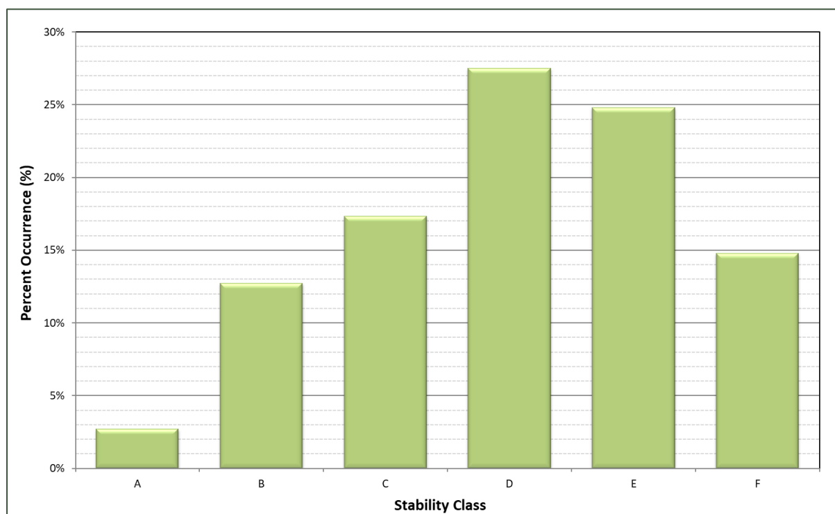
Figure 14 Stability Class as Predicted by CALMET (2016) at Girraheen FCS Site
