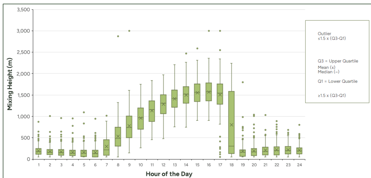
Figure 15 Mixing Heights as Predicted by CALMET (2016) at Girraheewen FCS Site
