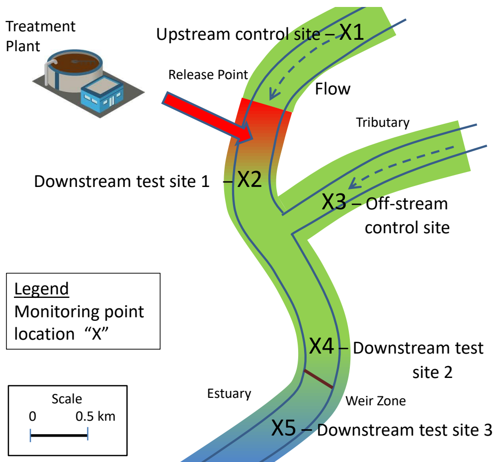
Figure 2. An example of a mid-field REMP, showing proposed locations for monitoring, for a sewage treatment plant release to a perennial freshwater stream.
